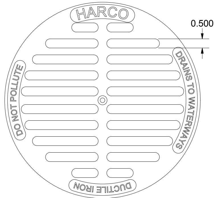
STANDARD 8" & 10" DROP-IN
